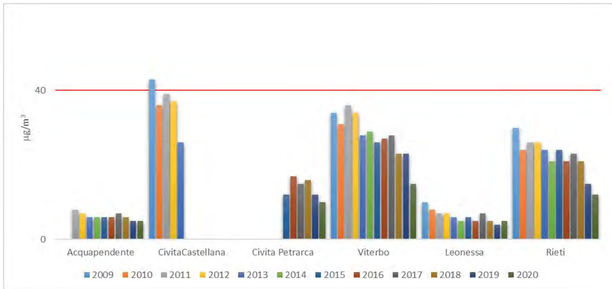
Figura 3-48 Media annua NO 2 zona Appenninica 2009-2020.
